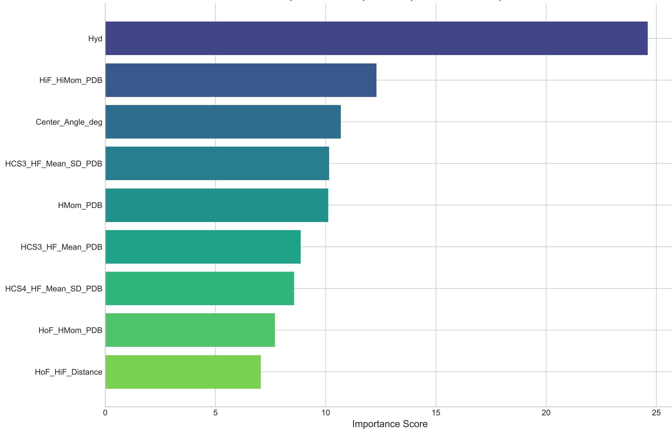
Top 9 Feature Importance (Two-Class Model)
